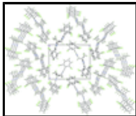
Fig. 2. The crystal packing of (I), viewed down the a axis, showing the molecules stacked along the a axis. Only the major disordered component is shown.
