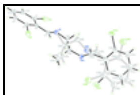
Fig. 1. The molecular structure of (I) with 50% probability ellipsoids for non-H atoms. All disordered components are shown.
